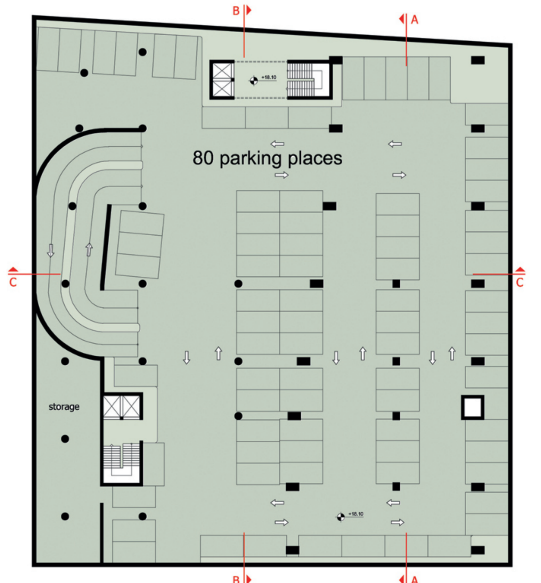
level -4 (+18.10)
