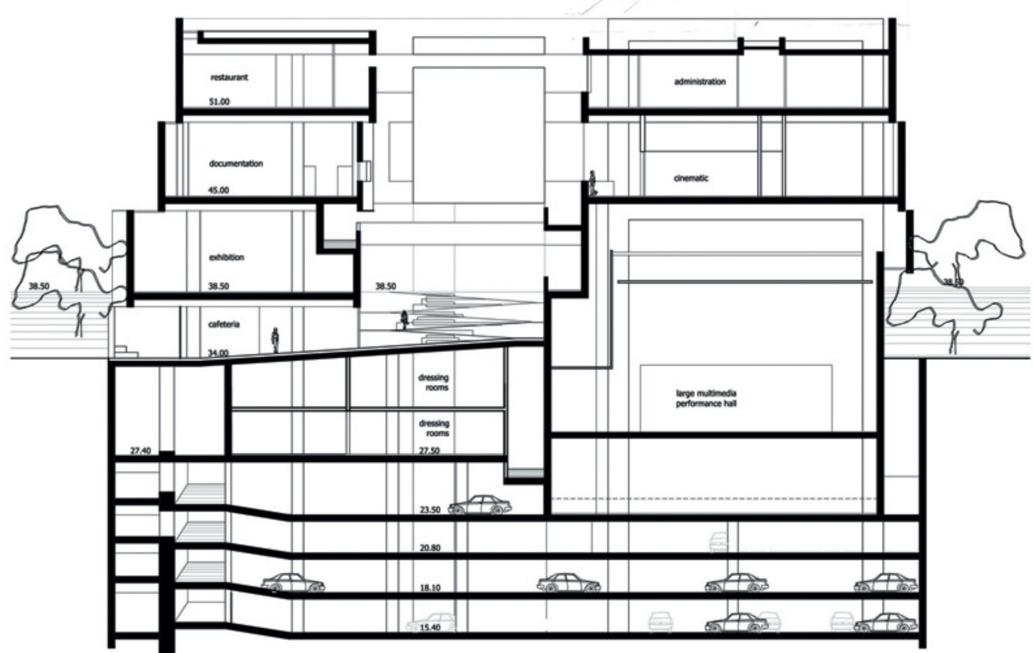
section c-c
