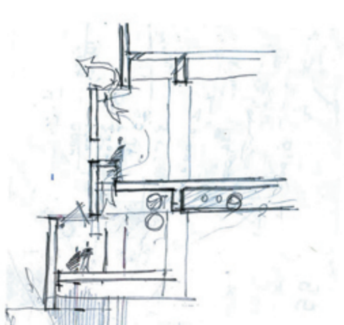
level 3 (+51.00)
